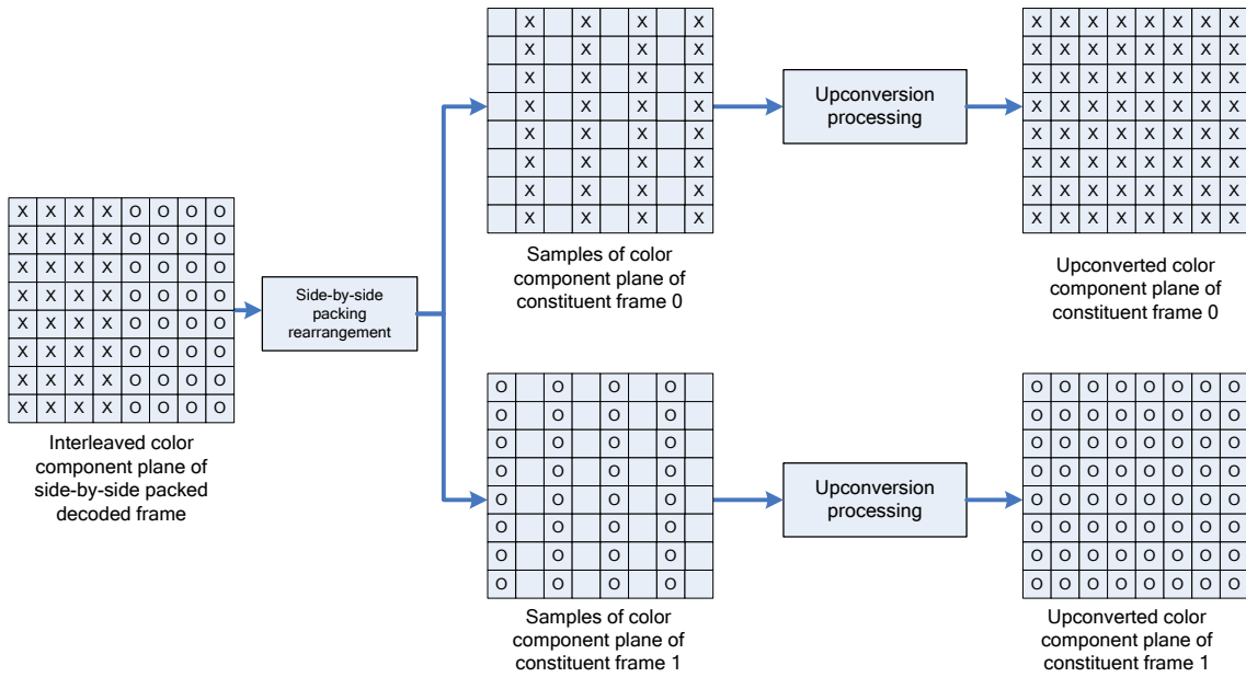
Figure D-7 – Rearrangement and upconversion of side-by-side packing arrangement with frame_packing_arrangement_type equal to 3, quincunx_sampling_flag equal to 0, and (x, y) equal to (12, 8) for constituent frame 0, and (x, y) equal to (0, 0) or (4, 8) for constituent frame 1
